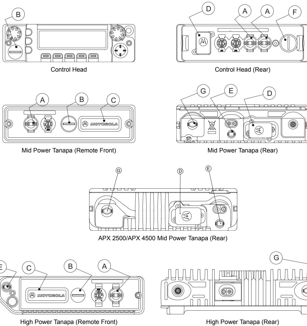
Figure 6-1. Dust Cover Installation Locations
