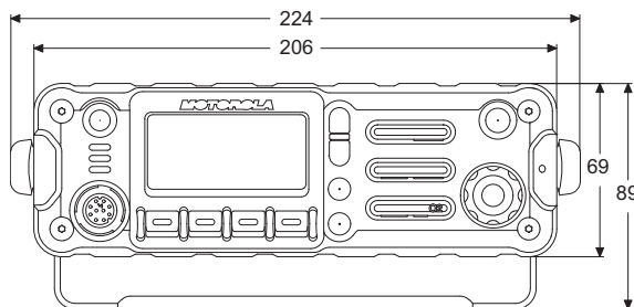
Figure 1-3. Front View of APX 2500/4500 Mid Power Dash Mount Transceiver and Trunnion
